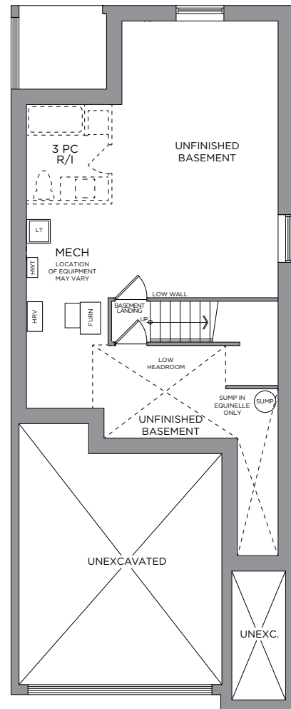
STANDARD BASEMENT
