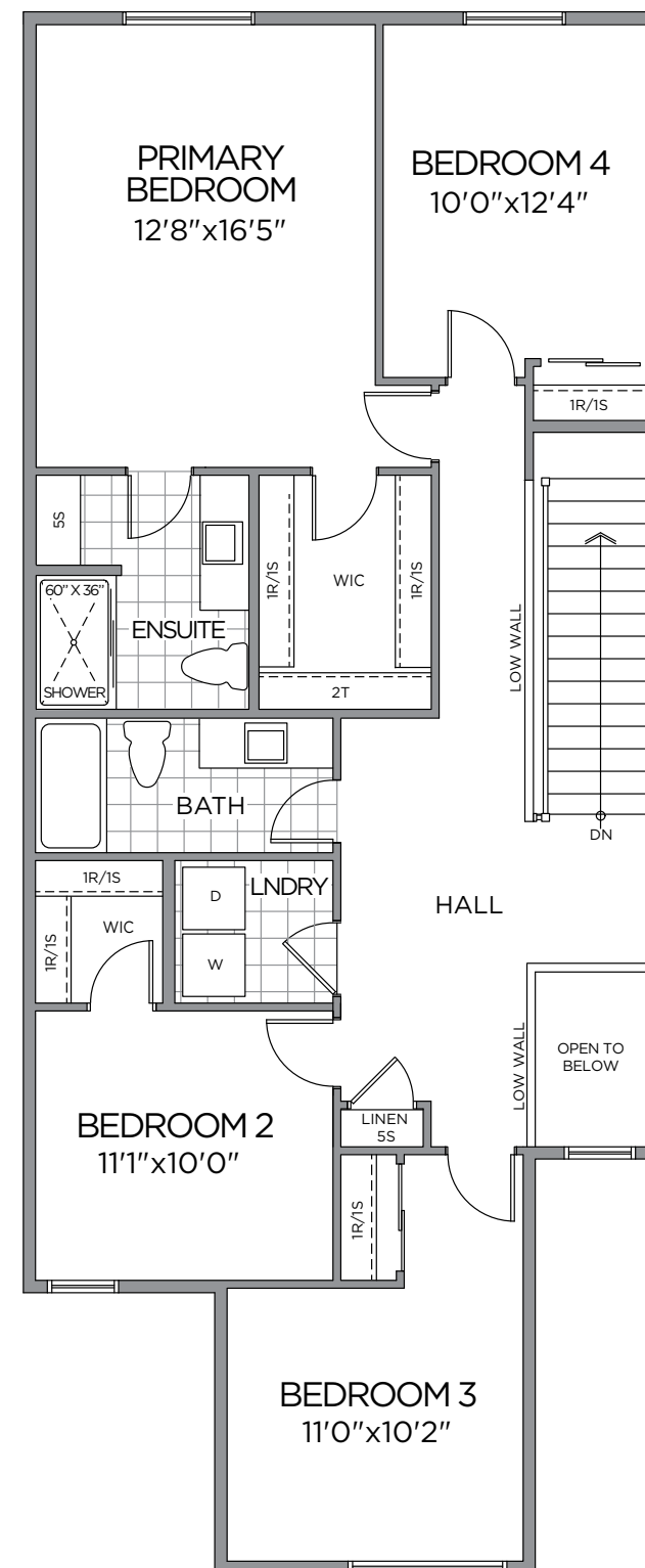
SECOND FLOOR
