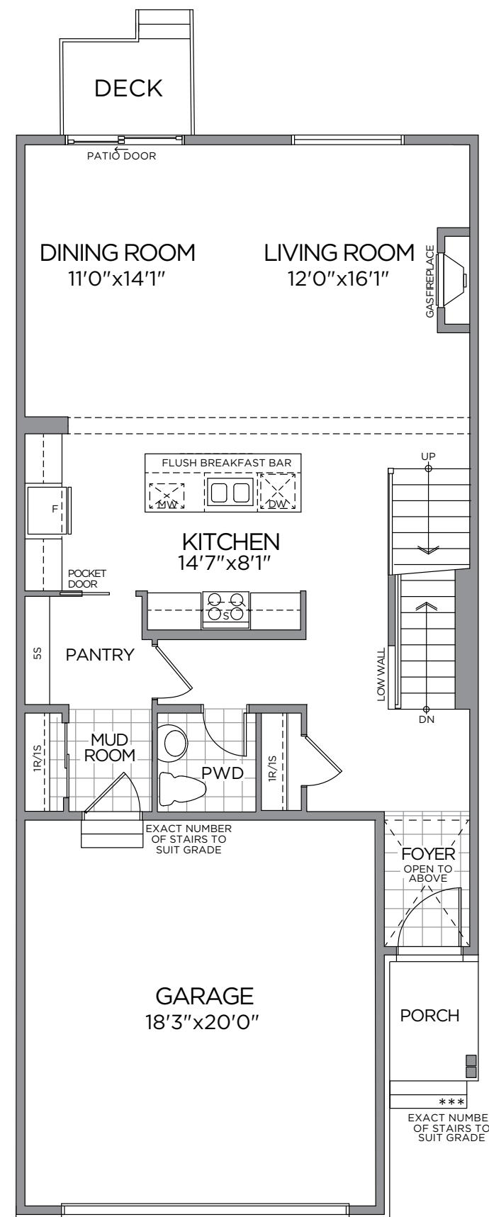
GROUND FLOOR
