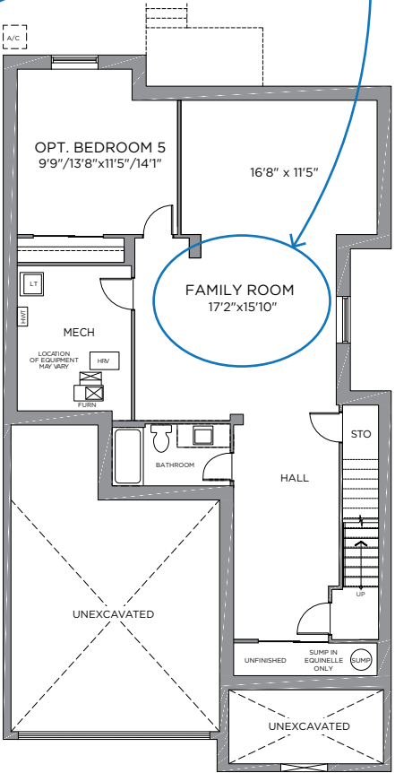
STANDARD BASEMENT FINISHED AREA 1074 SQ. FT.
