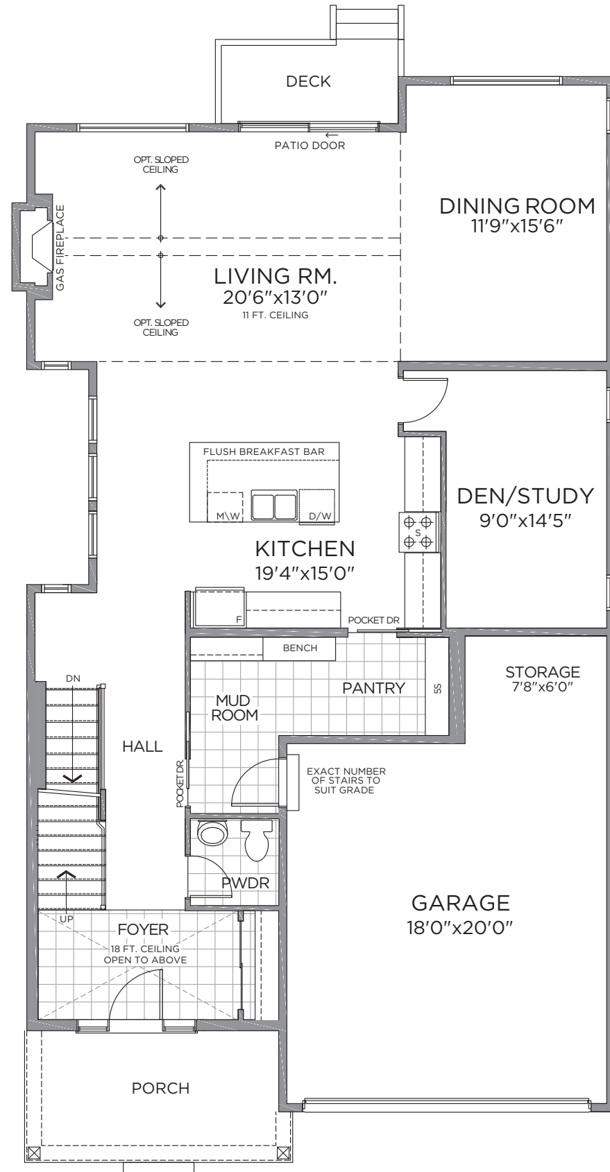
GROUND FLOOR ELEV. F
