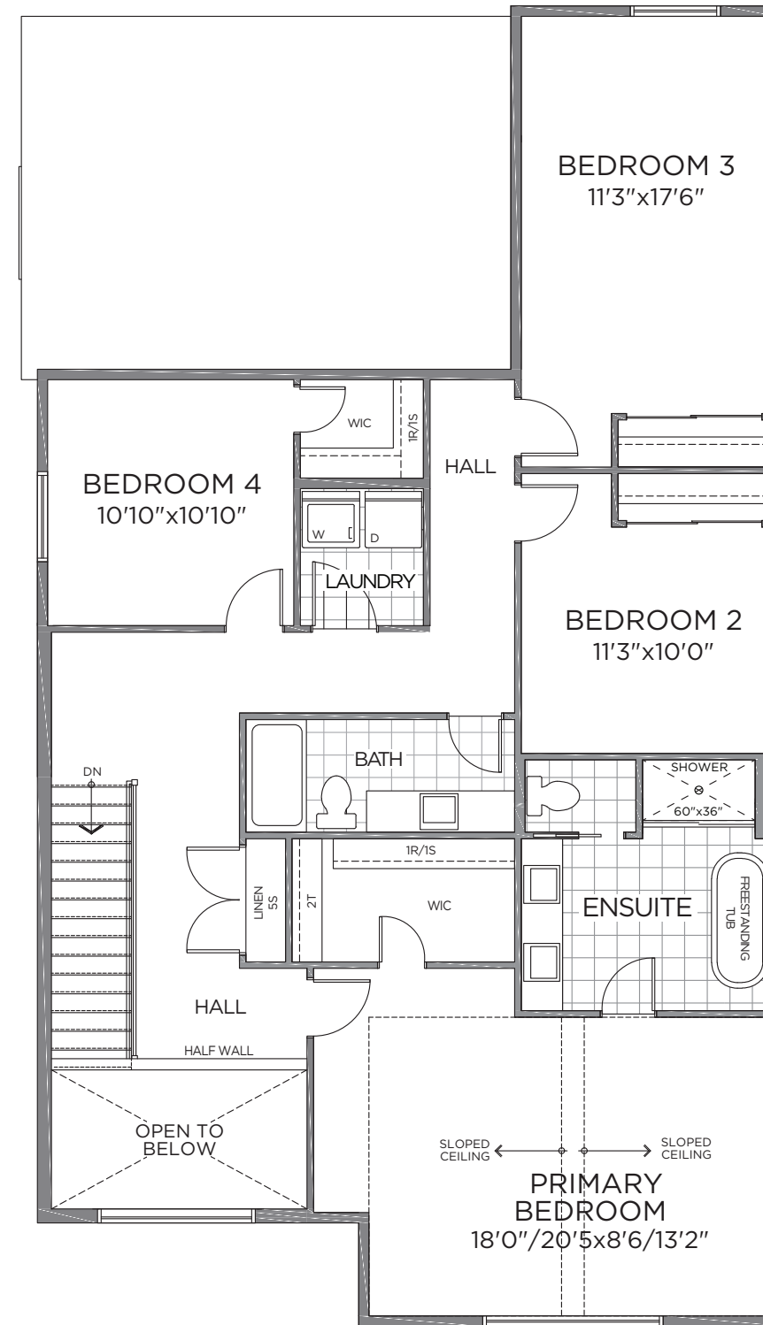
SECOND FLOOR ELEV. F
