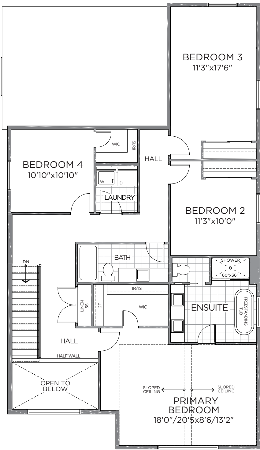
SECOND FLOOR
