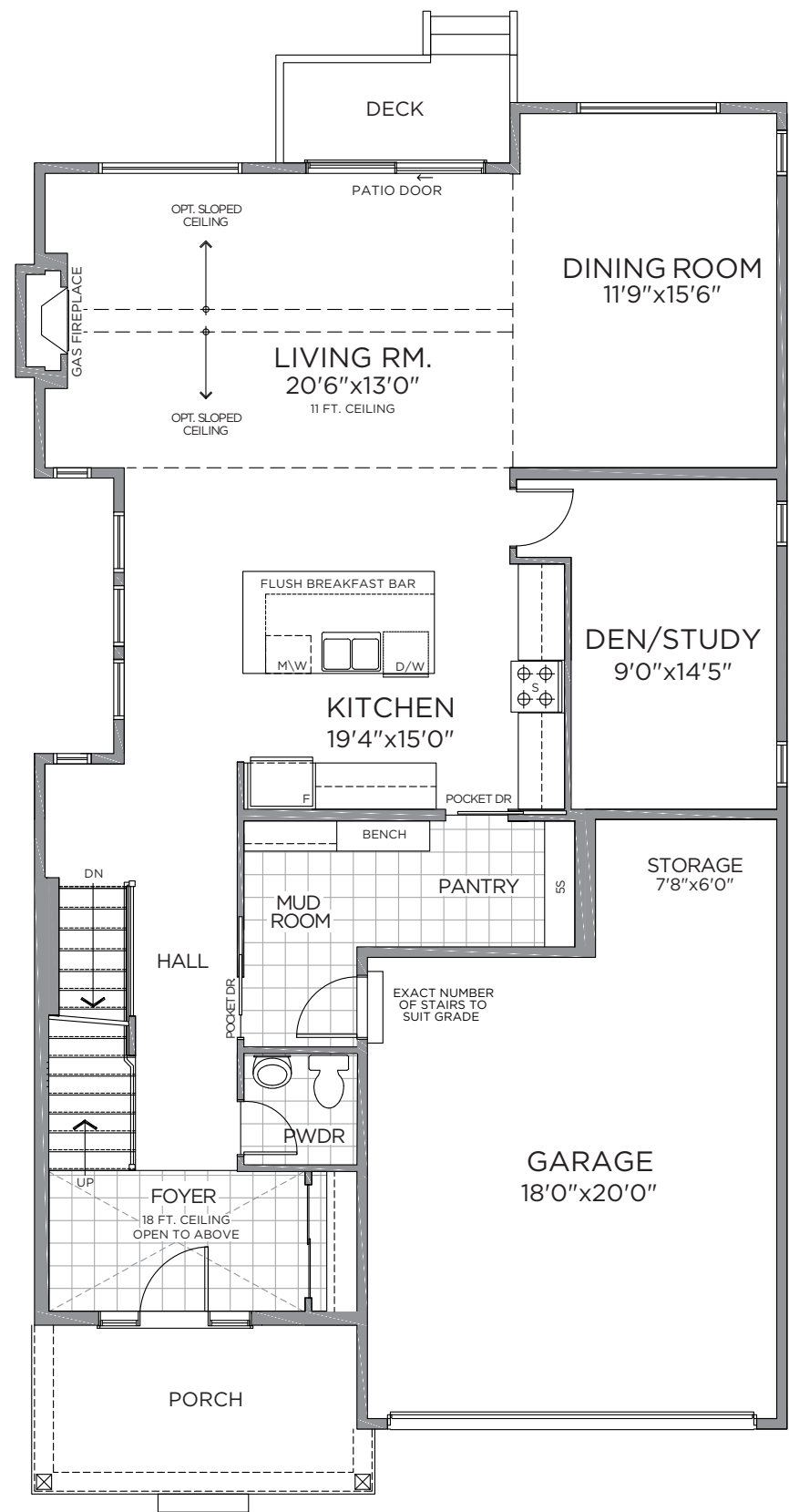
GROUND FLOOR
