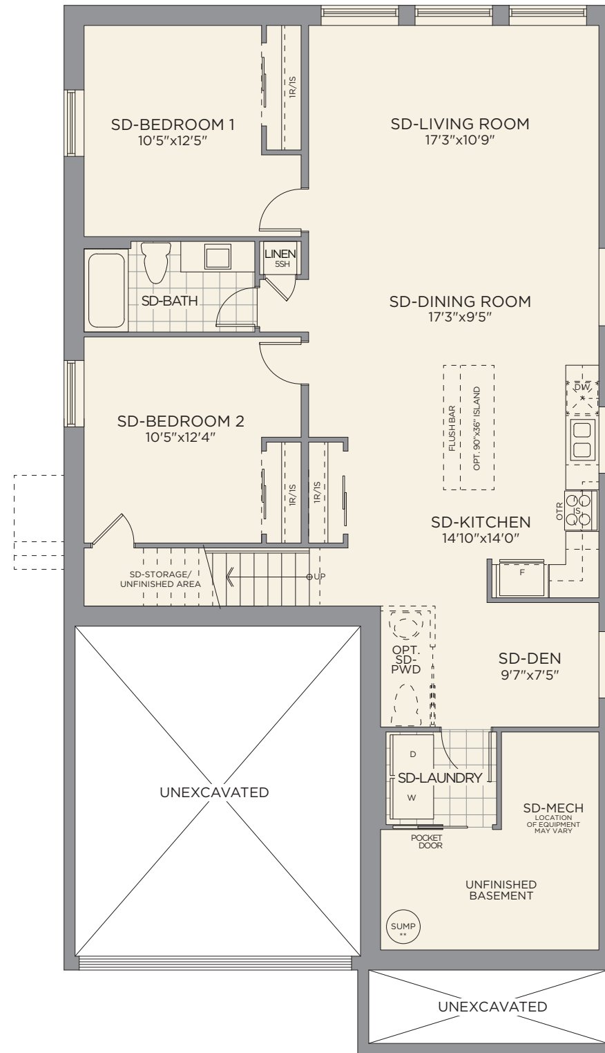
STANDARD BASEMENT PLAN (SECONDARY SUITE)
