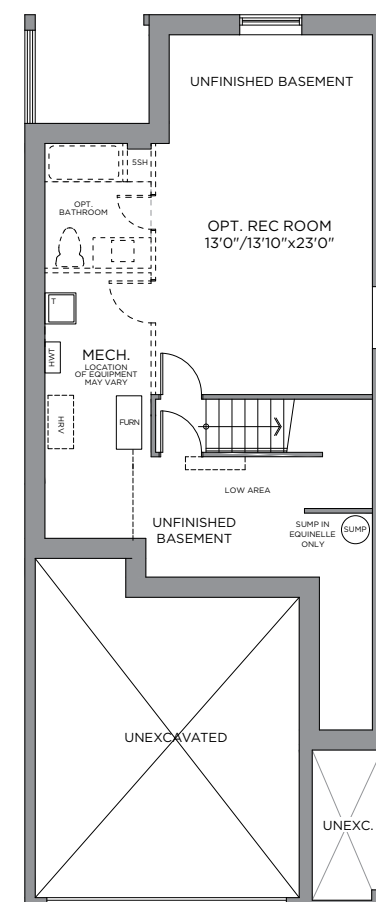
STANDARD BASEMENT ELEV. C OPT. FINISHED BASEMENT FINISHED AREA 468 SQ. FT.
