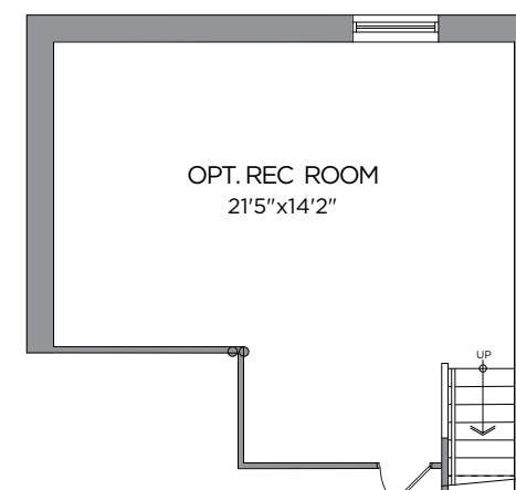
OPT. FINISHED REC. ROOM 434 SQ. FT.
