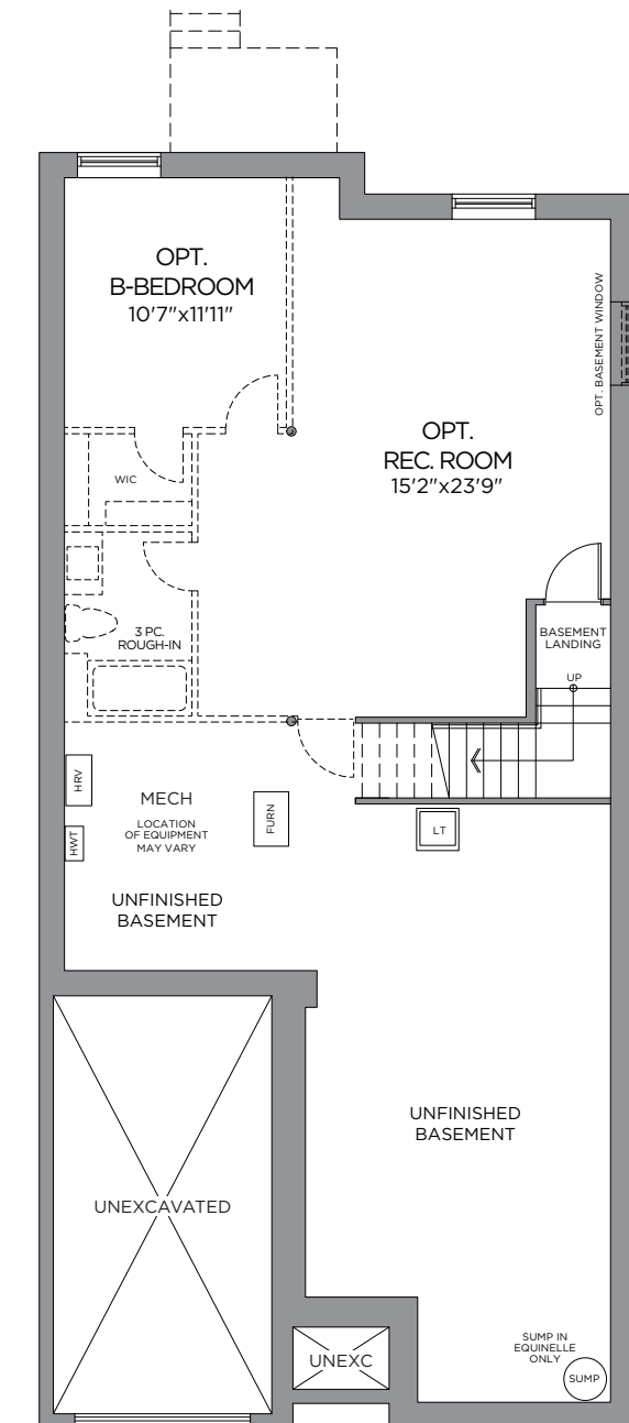
STANDARD BASEMENT OPT. FINISHED BASEMENT 750 SQ. FT.
