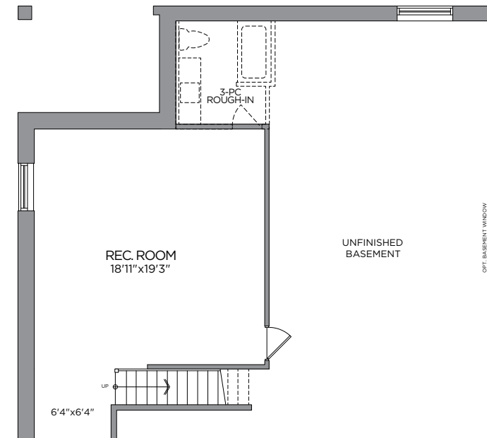
OPT. FINISHED BASEMENT REC. ROOM 477 SQ. FT.
