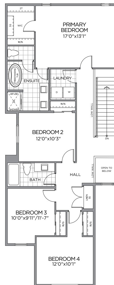
SECOND FLOOR PLAN OPT. PRIMARY ENSUITE PLAN
