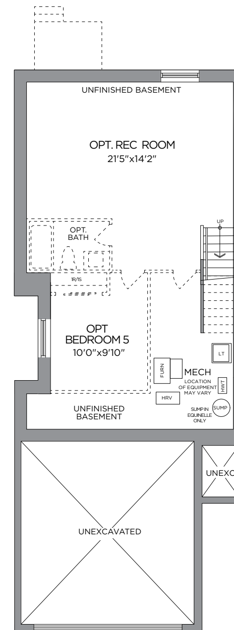
STANDARD BASEMENT PLAN OPT. FINISHED BASEMENT PLAN 636 SQ. FT.
